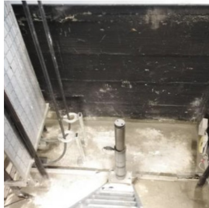
Elevator pit after waterproofing
